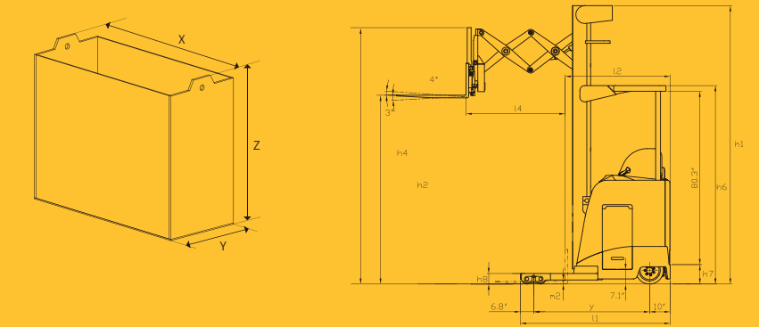
RATED CAPACITY AND LOAD DIAGRAM
