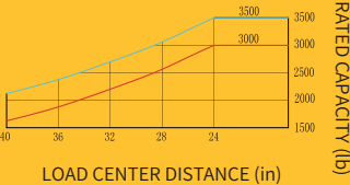
RATED CAPACITY AND LOAD DIAGRAM
